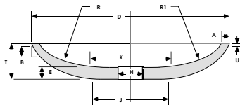
Type 99 Yates American Saw Grinder BP #1466
