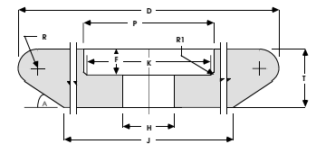
Type 5 Can-Car Chip 'N' Saw Grinder BP #26311
