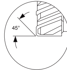
"M" lead-in (left hand helical flutes) may provide better penetration rates in steels over 200 BHN (only through hole)
