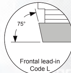
"L" lead-in may provide improved straightness. Reduce the feed by 40% of the values on pages 47-50 ("W" lead with chipbreaker)
