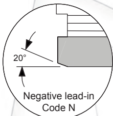
"N" lead-in is ideal for through holes. It is possible to increase the feed up to 100% of the values on pages 47-50
