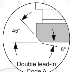
"A" lead-in can be used to improve finish
