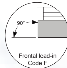
"F" lead-in can be used for stock removal at the bottom of the hole. Reduce the feed by 40% of the values on pages 47-50 ("Y" lead with chipbreaker)
