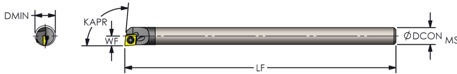
Carbide Boring Bar
