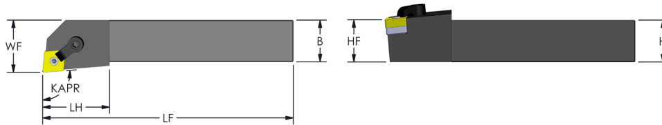
Negative 80° Diamond ( KAPR: 95°)
