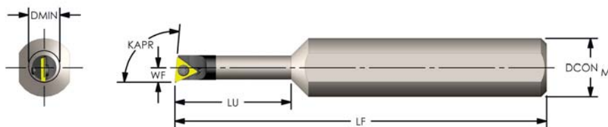
Positive Triangle (KAPR: 95°) Reduced Neck SERIES "F" Coolant Thru
