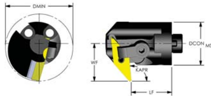
Negative 35° Diamond ( KAPR: 95°) Back Facing
