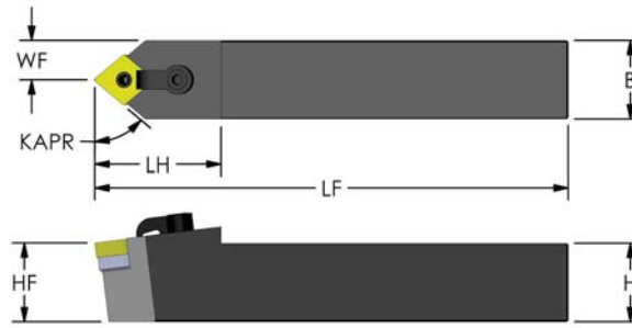
Negative 80° Diamond ( KAPR: 50°)
