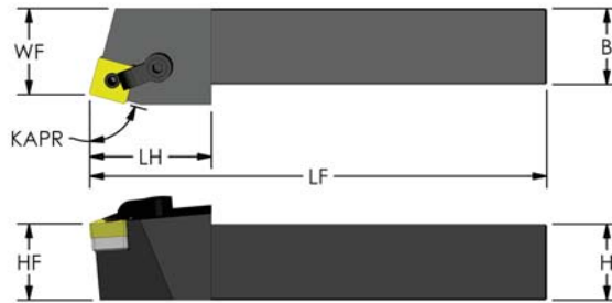
Negative Square (KAPR: 75°) Side Cutting
