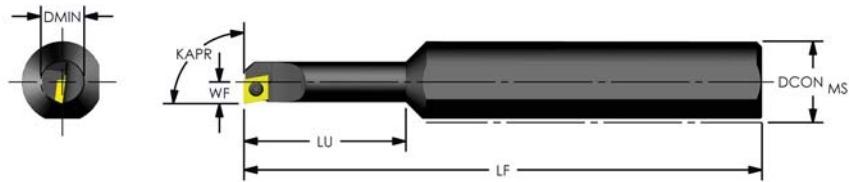
Positive 80° Diamond (KAPR: 90°) Reduced Neck
