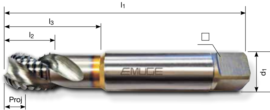
NPT Version shown • Semi-Bottoming Chamfer • TICN Coated
