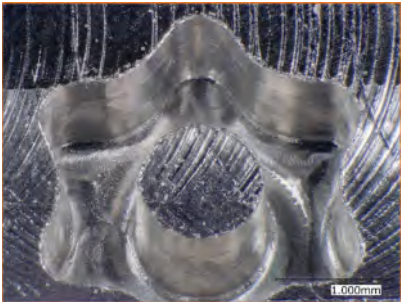
Burrs due to wear
