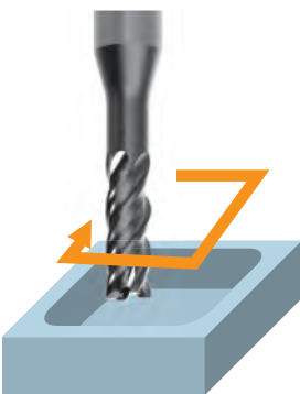
Pocket Milling
