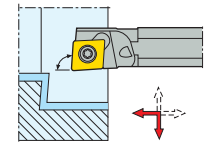
SCLCR/L, ..-R KAPR = 95,0 °
