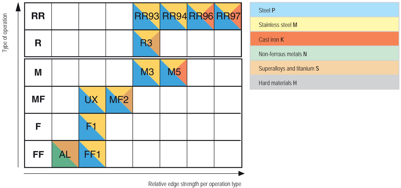
Chipbreaker chart for positive basic shape inserts
