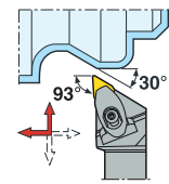
DDJNR/L...JETI KAPR = 93.0°
