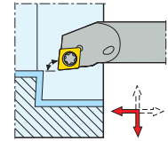
C.-SCLCR/L KAPRI = 95,0 °
