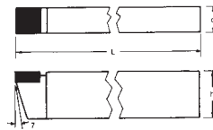
Turning/Facing Style C Square End
