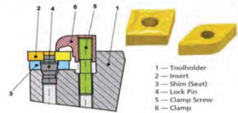
Combination Pin & Clamp "M" System
