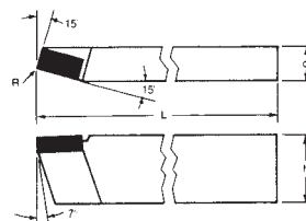
Turning Style B 15° Lead Angle
