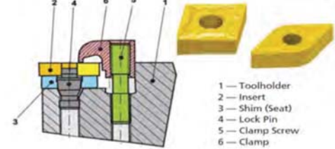
Combination Pin & Clamp "M" System
