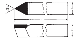
Threading Style E 60° Included Angle
