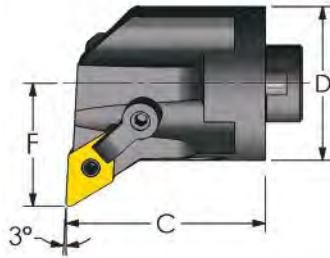
Negative 55° Diamond (-3° Lead) Coolant Thru
