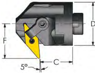
Negative 35° Diamond (5° Lead) Back Facing Coolant Thru
