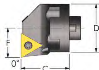
Positive Triangle (0° Lead) Coolant Thru
