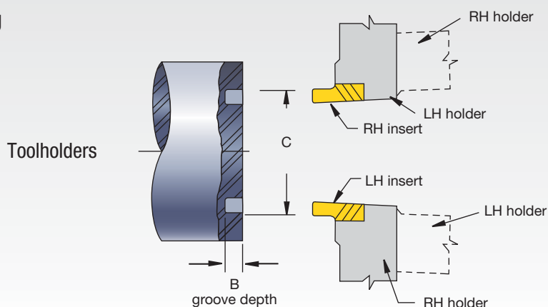
Standard NF/NDF Inserts
