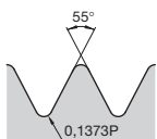
Whitworth BSW, BSP-External
