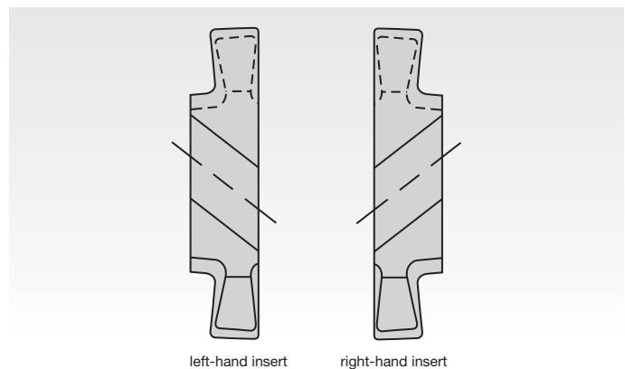
left-hand insert
