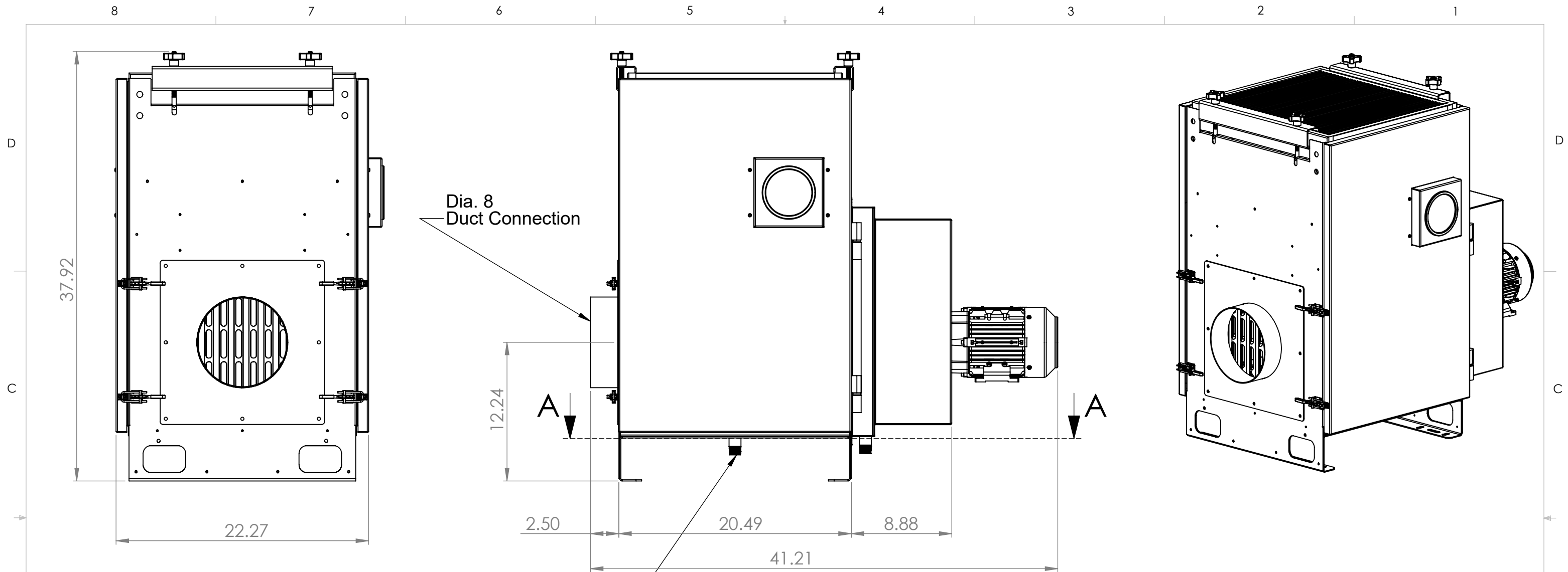
End View
