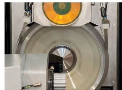
Agathon grinding machines equipped with PowerGrind technology
