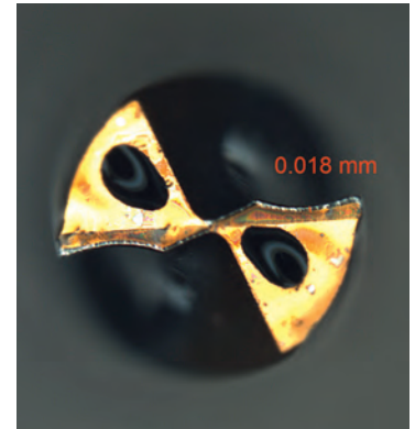
Tool wear <20 \mu\text{m} after 3421 holes
