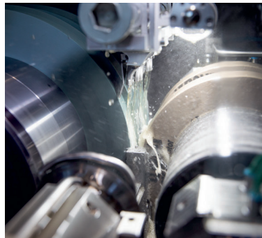
Centerless grinding (picture shows Tschudin proLine 400)
