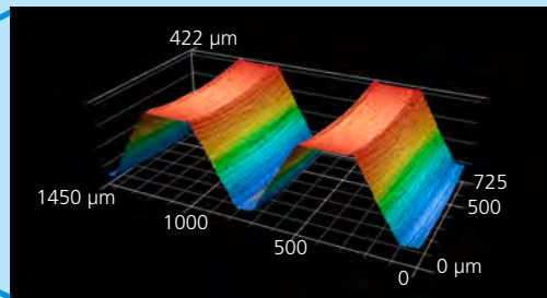
Vasco 601* Perfect thread profile
