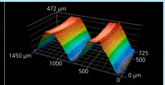
Standard coolant* Thread profile fails dimensional check
