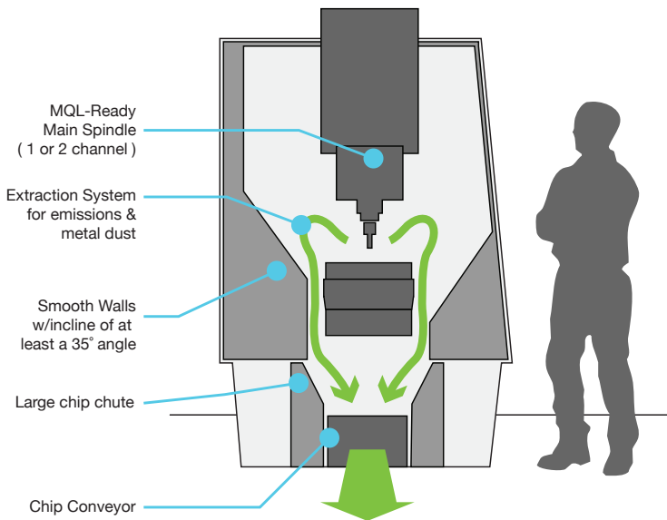
Figure 22: Elements of a MQL specific machining center
