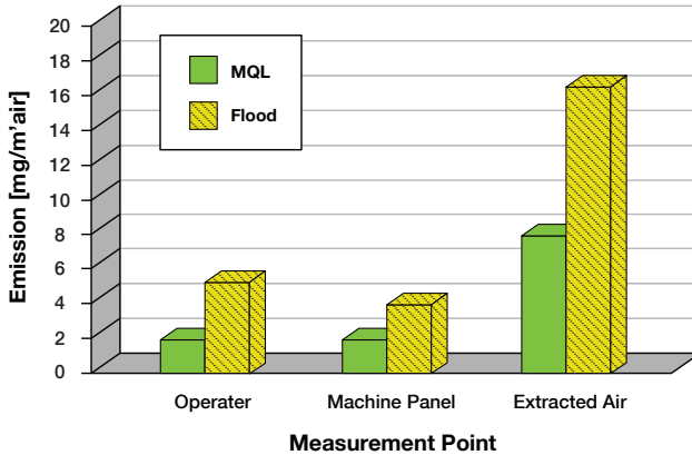
Figure 4: Comparing flood vs. MQL emissions
