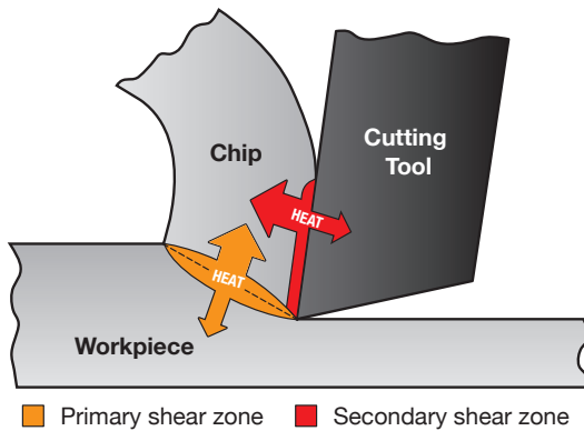
Figure 5: Heat generation in metal cutting
