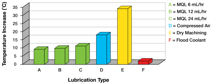
Figure 8: Temperature increase for different lubrication techniques
