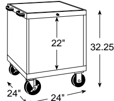
Mobile Housing No. 61209 Usable Height 22"
