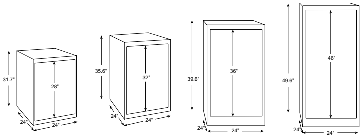
Housing No. 61300 Usable Height 28" Housing No. 61700 Usable Height 32" Housing No. 61400 Usable Height 36" Housing No. 61500 Usable Height 46"
