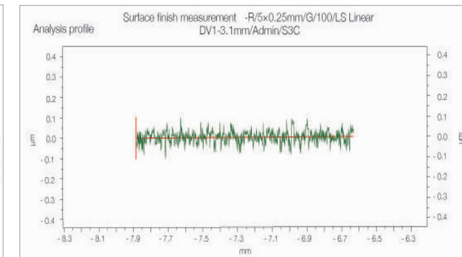
Surface Finish Measurement Data
