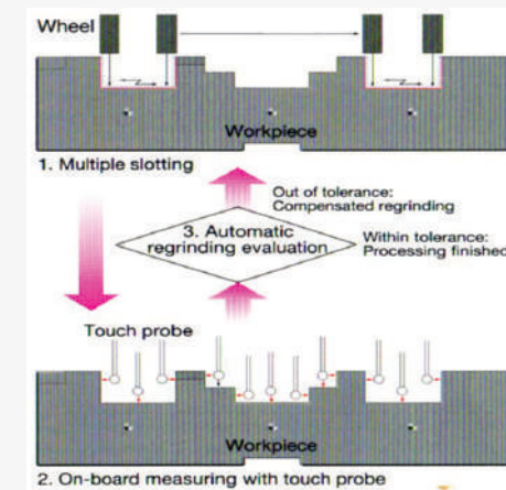
Programmable Measuring and Auto Re-Grinding
