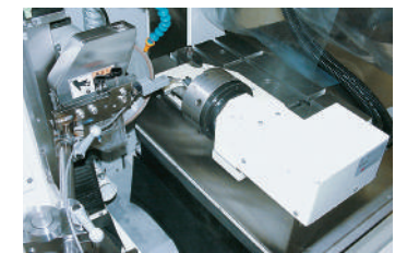
Tool Grinding Combining NC Swiveling Axis
