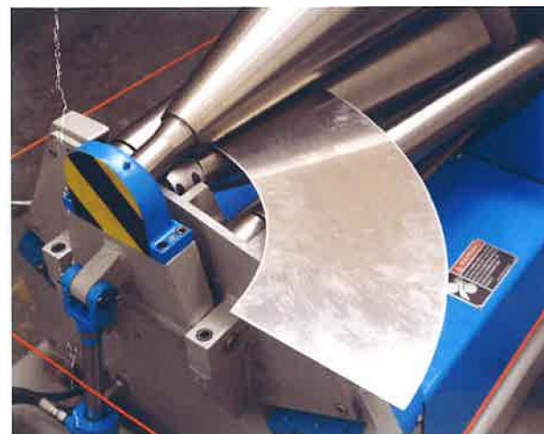
Work piece is entered into the machine & positioned via the calibrated pointer & gage roll.
