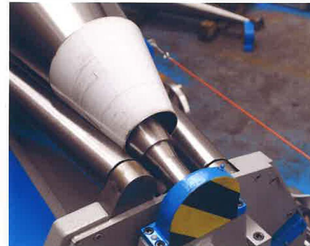
Rolls rotate to complete the forming cycle in 1 pass without any twist or edge deformation from a cone snubber (as with traditional rolls).
