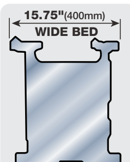
21 inch VS Lathe
