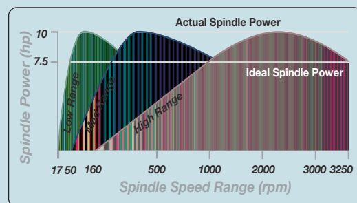
13 inch VS Lathe
