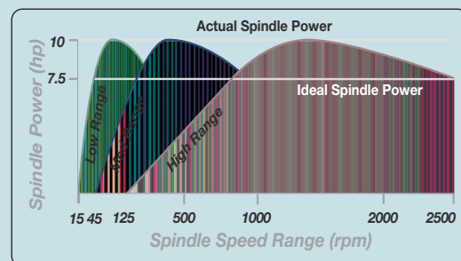
15 inch VS Lathe
