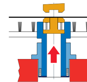
FORMING TOOL
