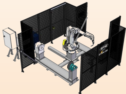
DT-ARC Dual Head/Tail Stocks
