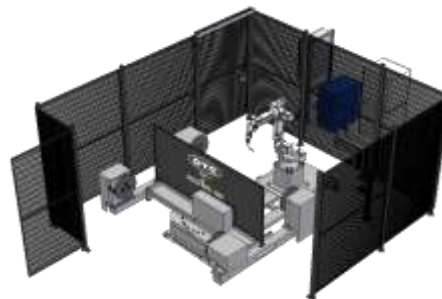
ROTA-ARC Pivoting Head/Tail Stocks
