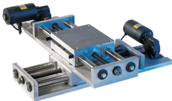
Welding Head Cross Slides
