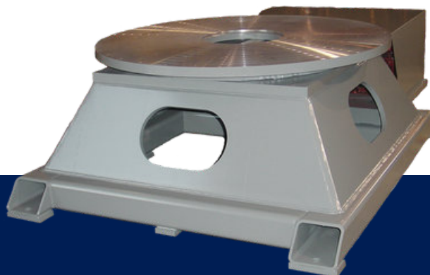
FT-400 40,000 lbs
