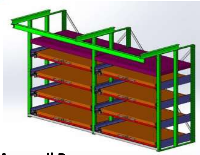
Integrated Monorail Beam
