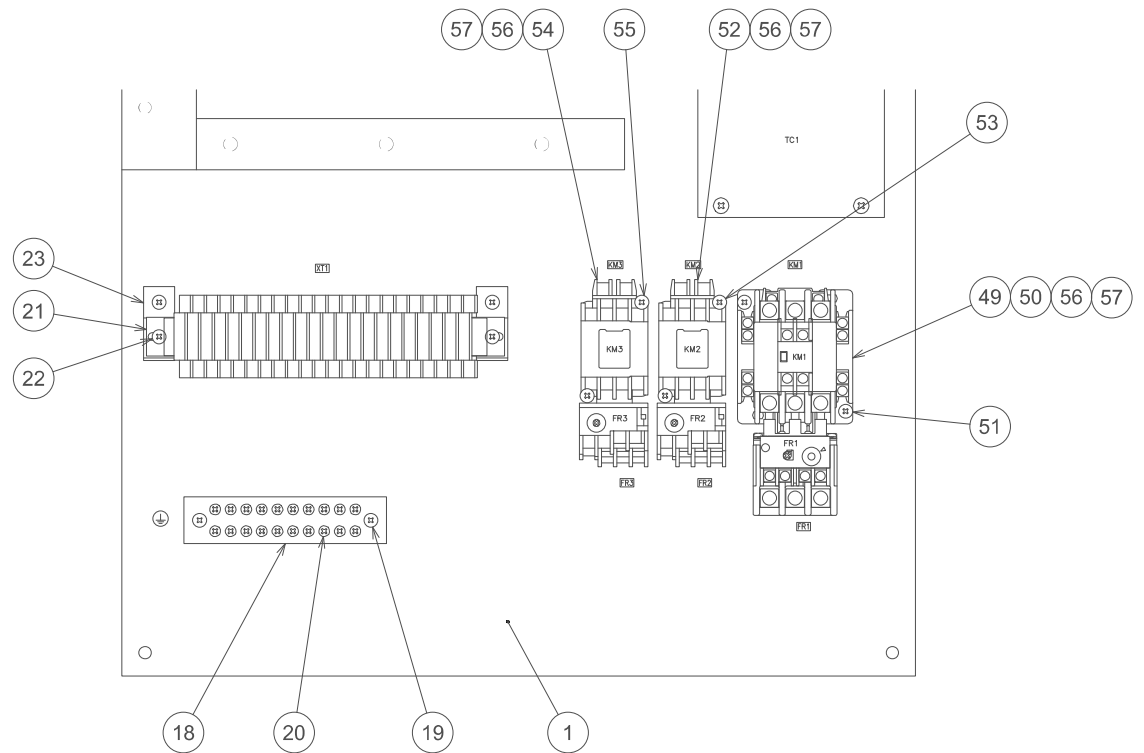
DETAIL B
