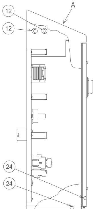
VIEW A
