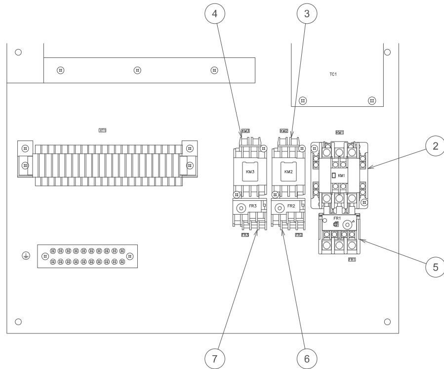
DETAIL B
