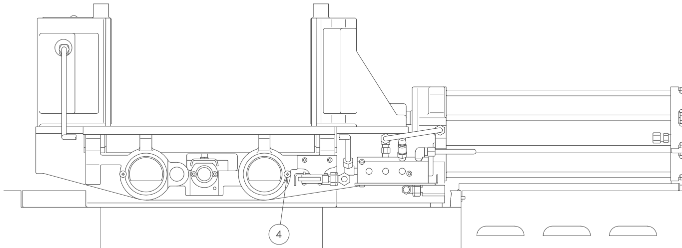
VIEW C
