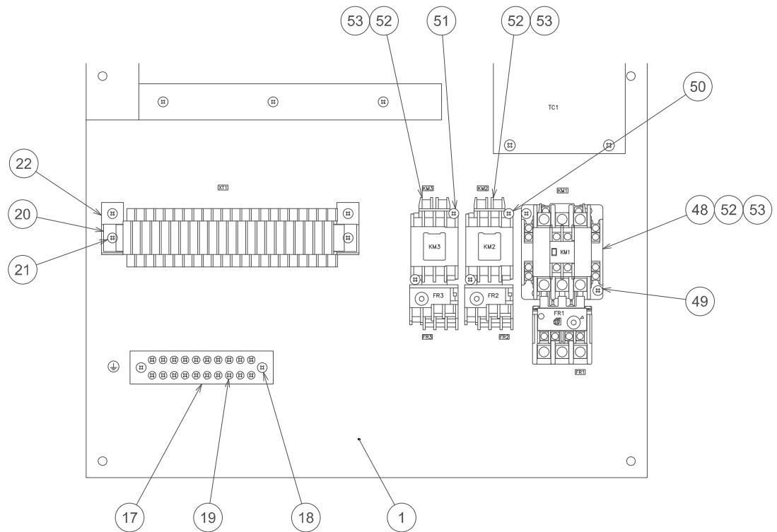
DETAIL B
