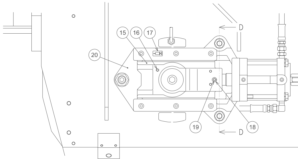
VIEW C
