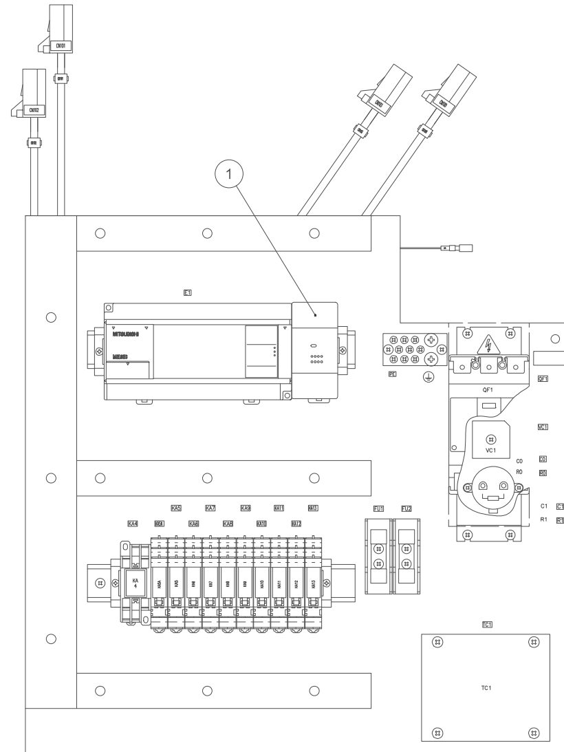
DETAIL A
