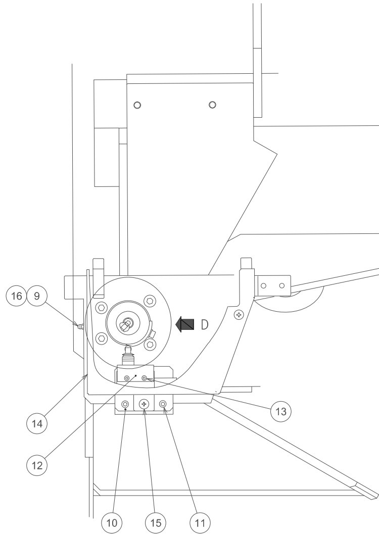
VIEW C
