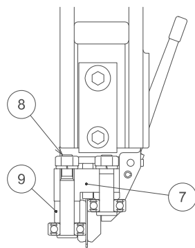
DETAIL C
