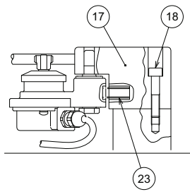
VIEW C
