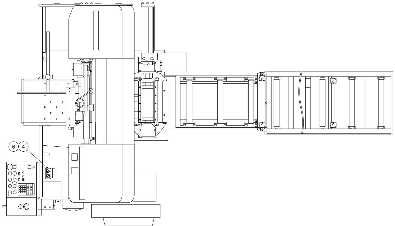
VIEW A
