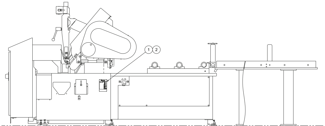
VIEW B
