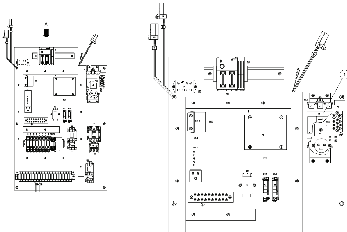
DETAIL A
