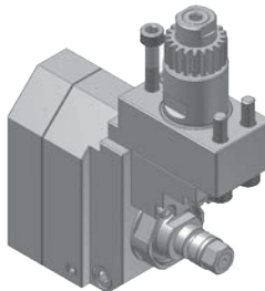
HWX731000 Slotting unit
