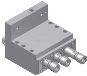
NUB261100 3 spindle drilling/milling unit
