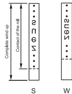
Marking types on work piece
