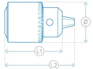
Jacobs Taper or Threaded Mount
