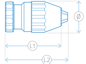
Jacobs Taper or Threaded Mount
