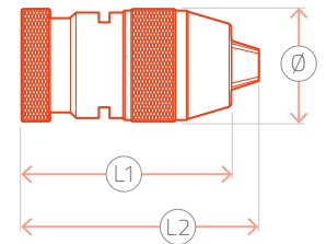
Jacobs Taper
