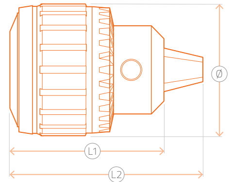
Jacobs Taper
