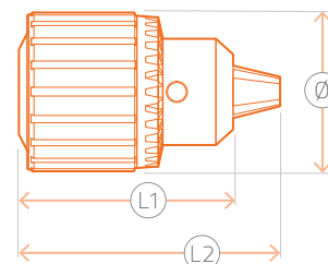
Jacobs Taper or Threaded Mount
