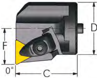
PULLBACK Clamp Negative Triangle (0° Lead) Coolant Thru
