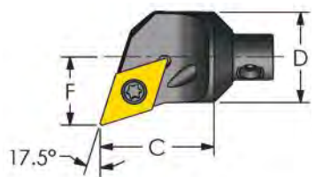
Positive 55° Diamond (-17.5° Lead) Profiling Coolant Thru
