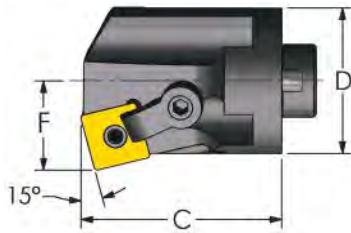
Negative Square (15° Lead) Coolant Thru
