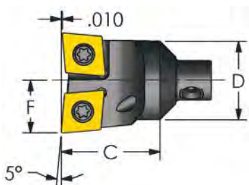
Positive 80° Diamond (-5° Lead) Turn & Bore Coolant Thru
