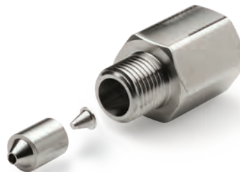
MA-FIL-06 $170 1/4" F to 1/4" M Diamond Guard Filter Assembly MA-FIL-06NF $55 1/4" F to 1/4" M DGF Body & Insert (No Filter)
