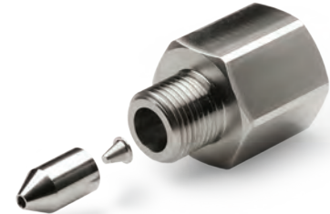
MA-FIL-08 $185 1/4" F to 1/4" M 90K PSI Diamond Guard Filter Assembly MA-FIL-08NF $70 1/4" F to 1/4" M 90K PSI DGF Body & Insert (No Filter)
