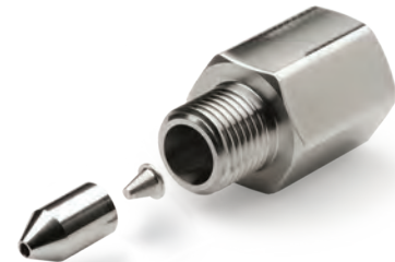
MA-FIL-M-09 $185 M16 F to M16 M Diamond Guard Filter METRIC M16-1.5 Threads MA-FIL-09NF $70 M16 F to M16 M DGF Body & Insert (No Filter) METRIC M16-1.5 Threads
