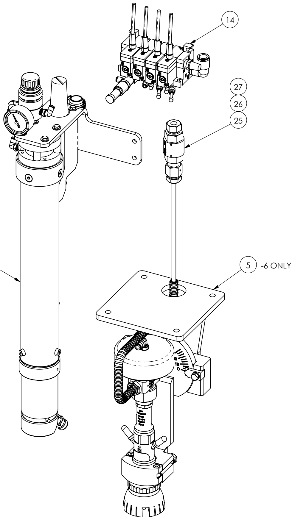
CUTTING HEAD KIT - CWJ MANUAL TILT 060068-6
