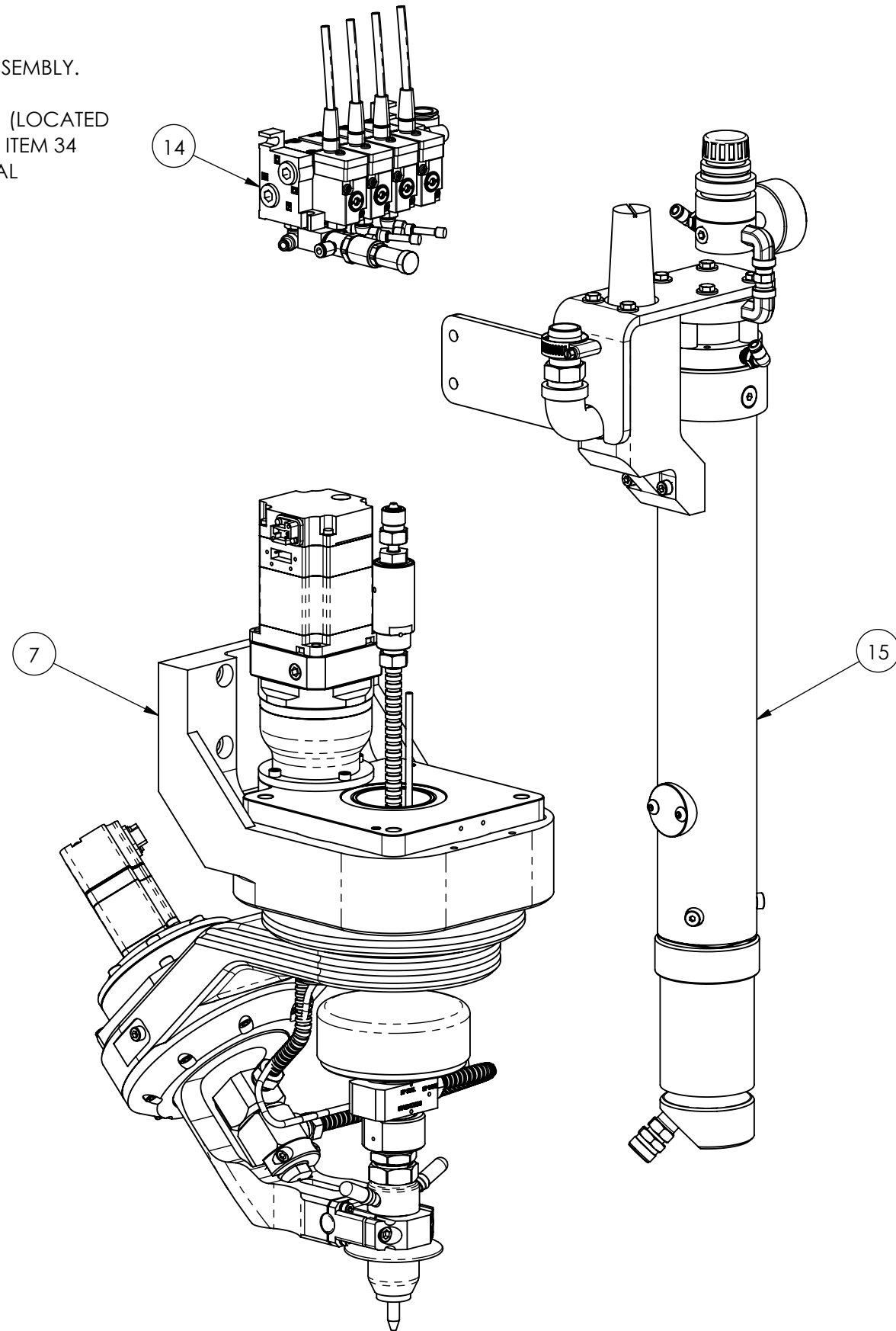
CUTTING HEAD KIT - M200 PIVOT PLUS 060068-7
