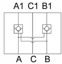
Circuit drawing
