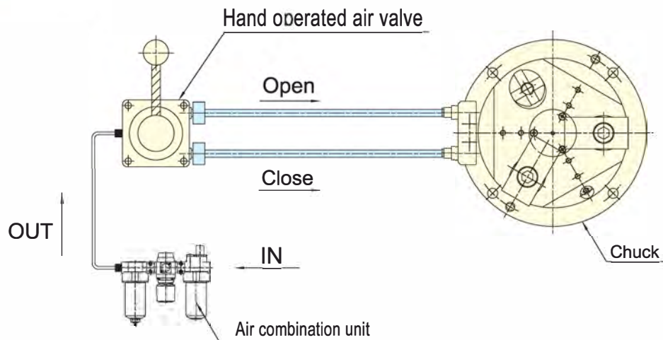
Assembly drawing
