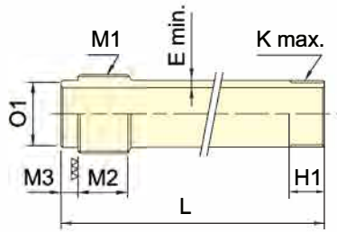
Detail of Draw Pipe L=A+G2max.+H-G1max.+M2+M3
