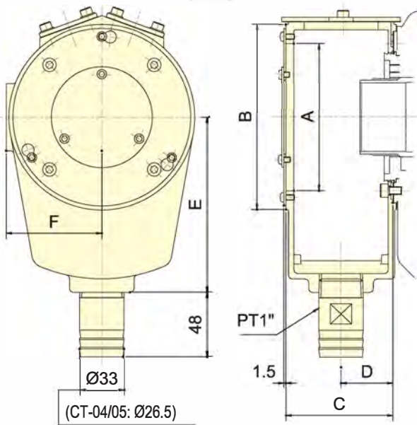
Coolant Collector
