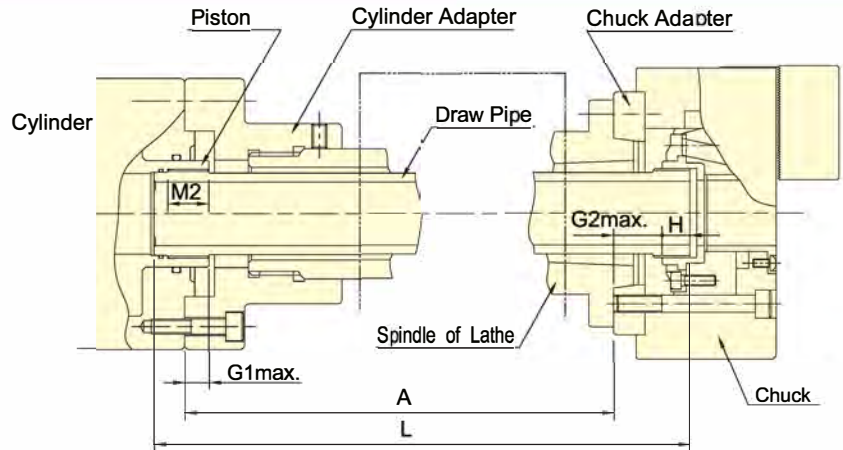
Detail of Draw Pipe L=A+G2max.+H-G1max.+M2+M3
