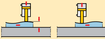
Figure 8 Hydraulic clamping
