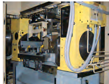
Synchronors movement of 2 off CNC401
