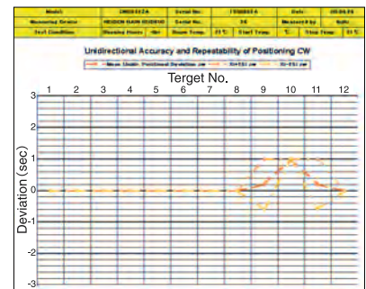
Unidirectional Accuracy and Repeatability of Positioning
