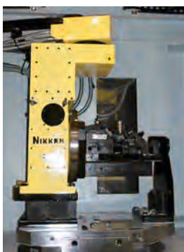
Photo shows CNC302T without T slot.
