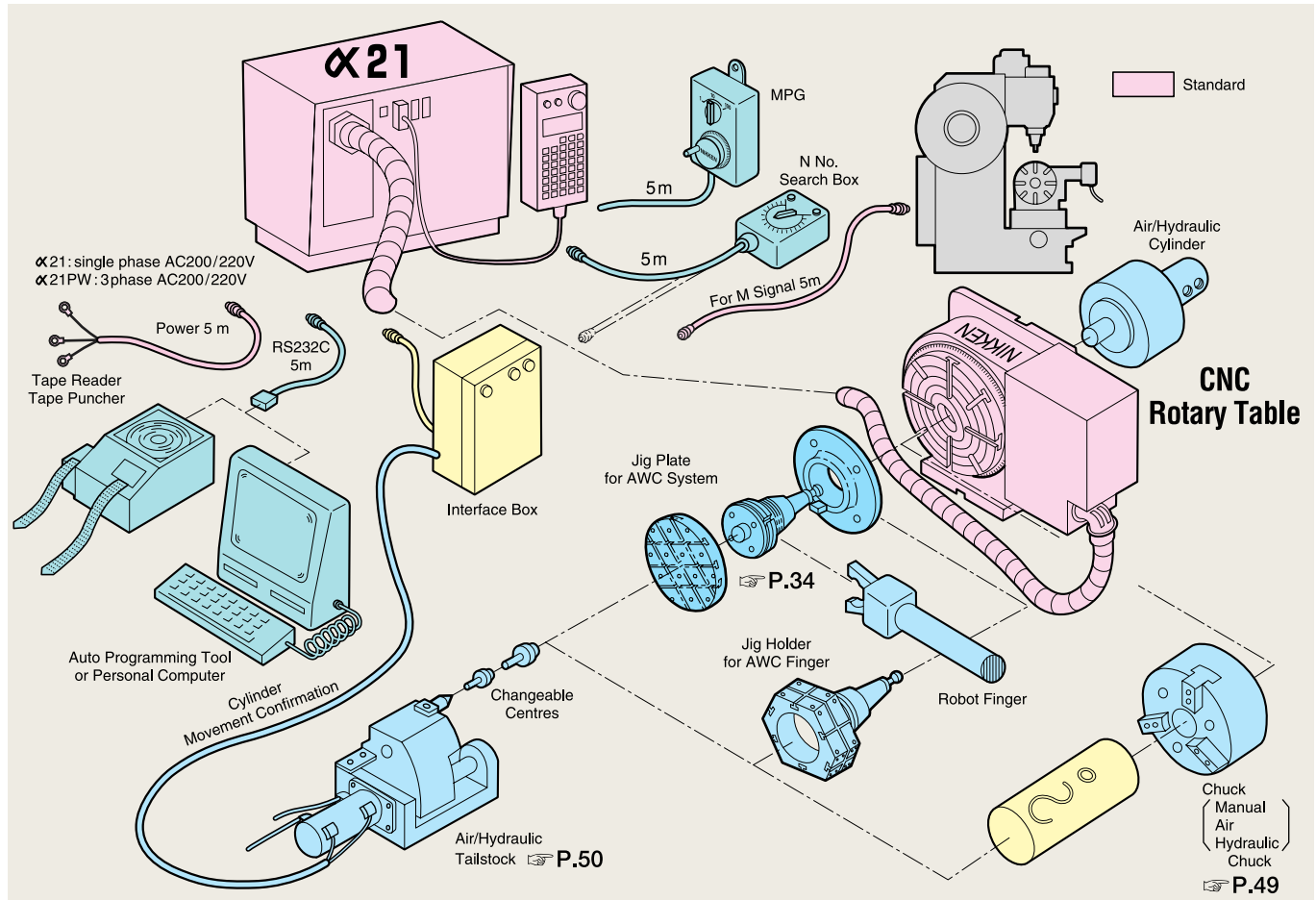
Ø21 controller for larger capacity (2.7KW, 4.4KW and 11kW) is available. • 3 phase AC200/220V
