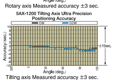
Tilting axis Measured accuracy ±3 sec.
