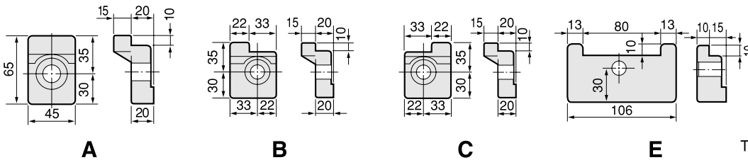
T-slot pitch guide piece
