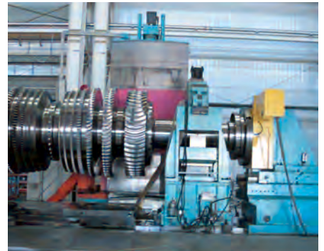
Indexing of the turbine shaft
