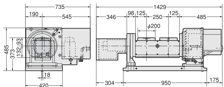
5AX-2MT-200-250
