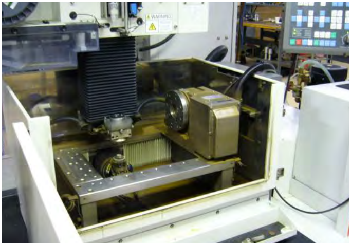
Wire EDM
