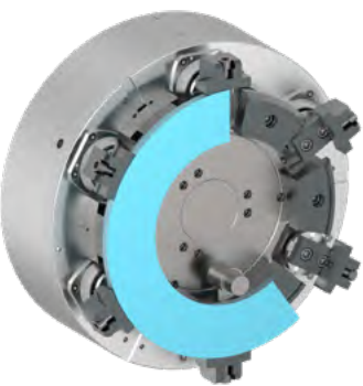
Chuck jaws for O.D. clamping – OP10
