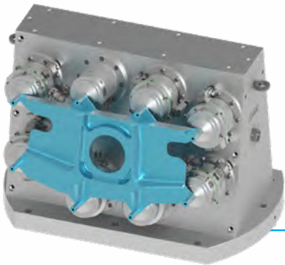
Clamping of titan pintel plate VERO-S
