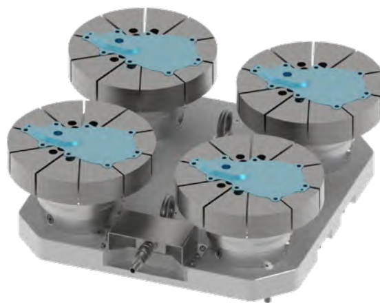
VERO-S fixture membrane with active pull-down
