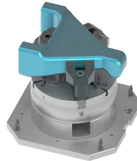
Manual 3-jaw chuck ROTA-S plus 630 with quick-change jaws
