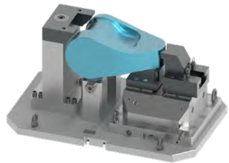
Clamping force block TANDEM
