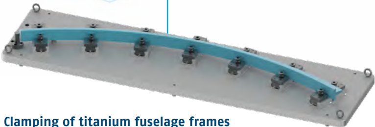
Clamping of titanium fuselage frames KONTEC vises solutions
