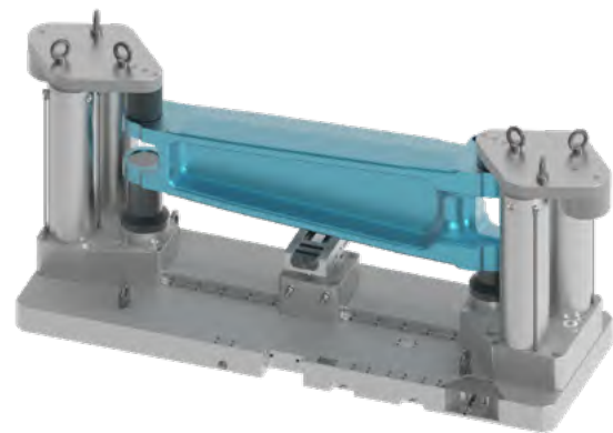
Hydraulic expansion arbor and VERO-S
