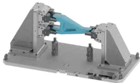
Clamping forces block TANDEM KSP 160
