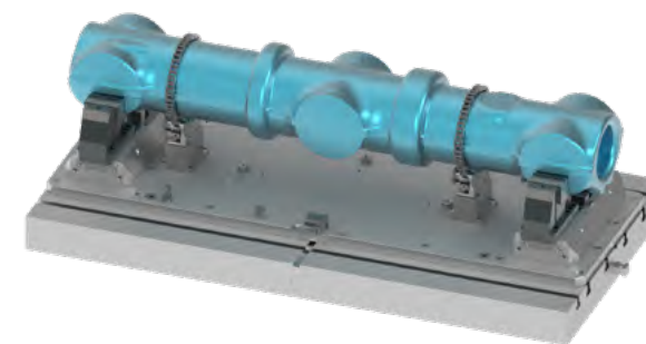
Clamping force block TANDEM KSP3 315
