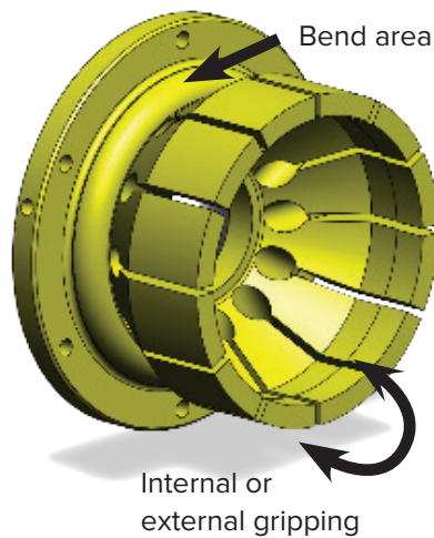
B-36827 External Gripping Finger Chuck
