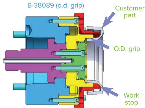
External finger chuck Drawbar actuation
